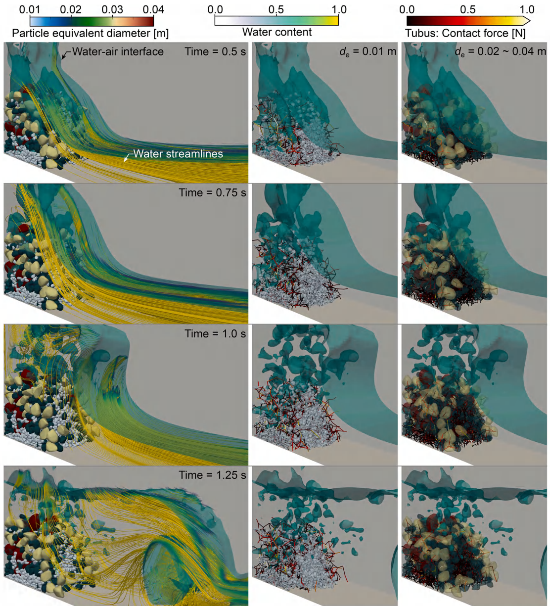
(a) Initial impact of dam-break wave (b) Contact networks of fines (c) Contact networks of coarse particles
