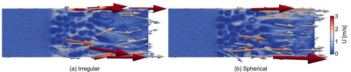
Fig. 25. Fluid velocity field for different shapes of coarse grains: (a) irregularly-shaped case and (b) spherical case.
