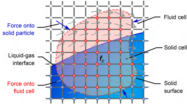
Fig. 2. Illustration of resolved CFD-DEM coupling. Particle boundaries are explicitly resolved by the fluid mesh, and fluid-particle interaction is computed via direct stress integration over particle surfaces.
