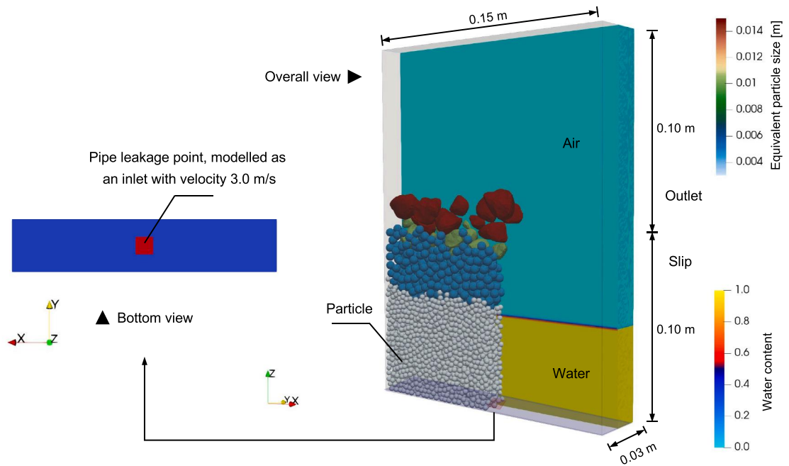
Fig. 35. Model setup for simulating the jet-induced destabilization in granular media. The fluid and particle domains are visualized using half-section views along the y - and x -axes, respectively.
