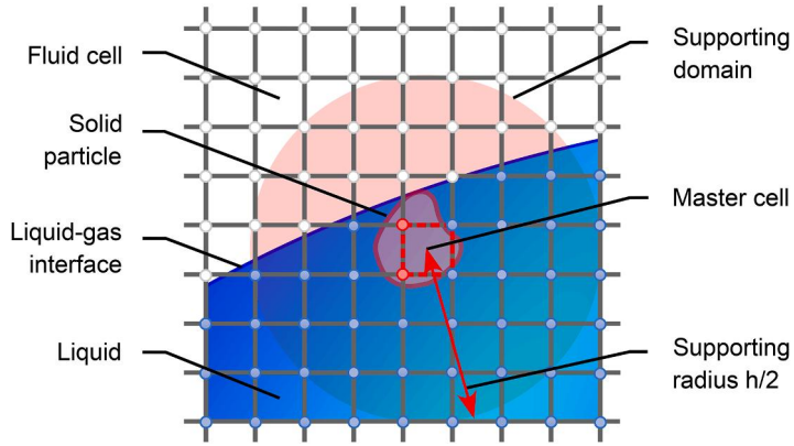
Fig. 4. Illustration of semi-resolved CFD-DEM coupling. Moderately sized particles interact with multiple fluid cells. Fluid properties are interpolated from surrounding cells using a kernel function, and interaction forces are conservatively spread back to the fluid grid.
